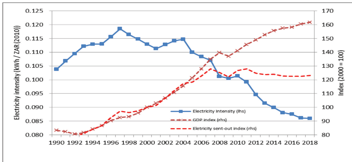
Figure 4: Electricity Intensity History 1990–2016 (Source: Own Calculations based on Statistics SA Data)
